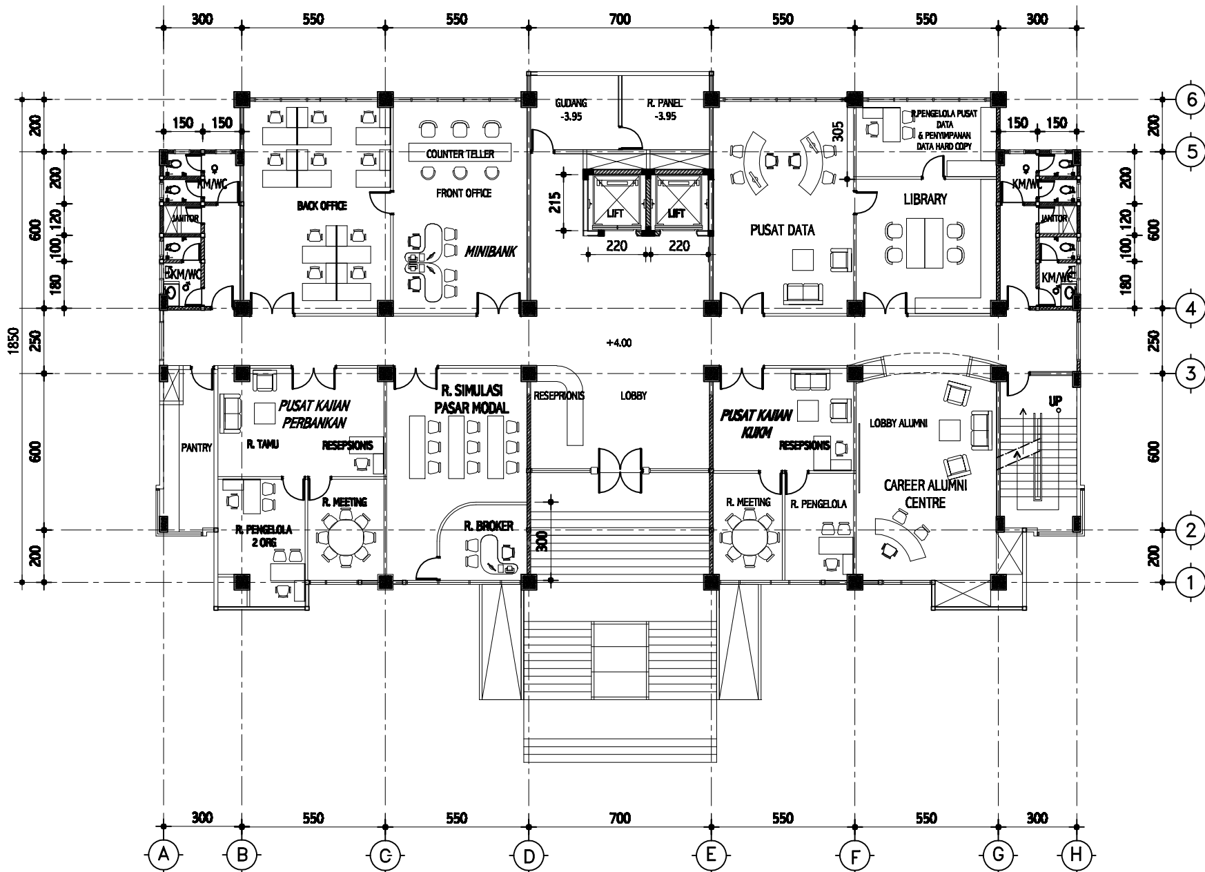
DENAH LT. 01
